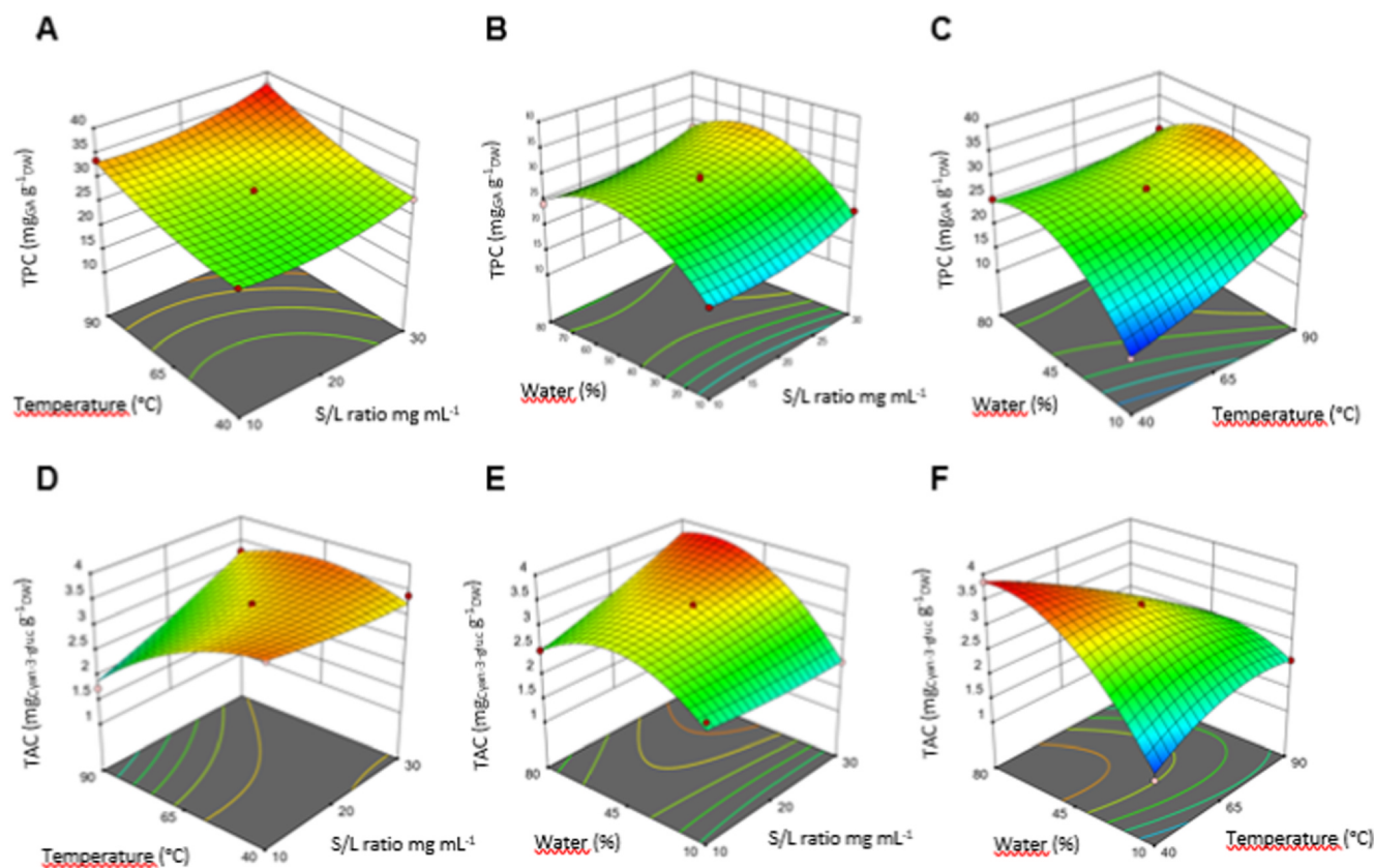
Fig. 1. 3D response surface representations for interaction of three tested extraction variables on the total phenolic content, TPC (A–C) and total anthocyanin content, TAC (D–F).
