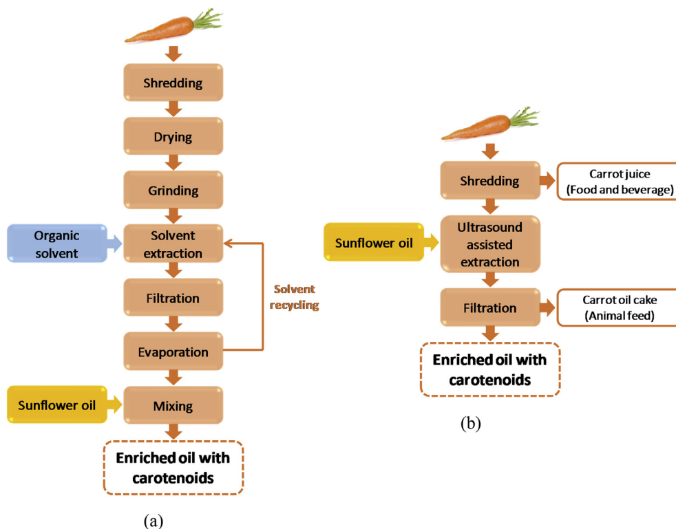
Fig. 6. Processing procedures to obtain enriched oil with carotenoids by (a) conventional solvent extraction and (b) ultrasound assisted extraction.
