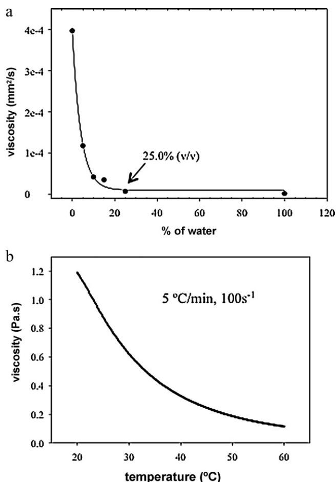
Fig. 2. Relationship between (a) viscosity and added water percentage (v/v), (b) viscosity and temperature of glucose–choline chloride–water (2:5:5, molar ratio).
