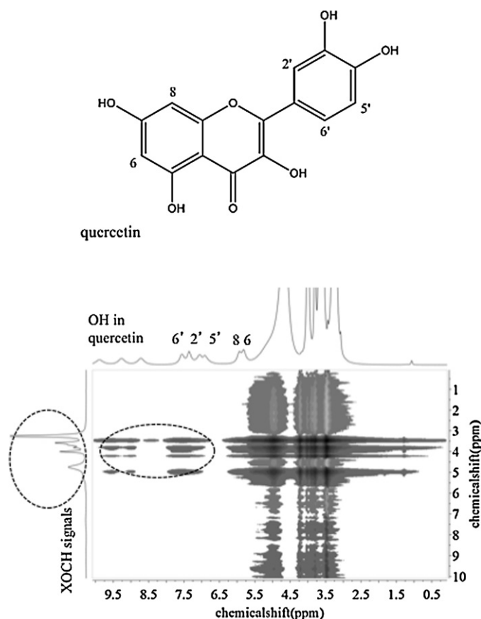
Fig. 4. 1 H– 1 H-nuclear overhauser enhancement spectroscopy of correlation between solute (quercetin) and xylitol–choline chloride–water (XoCH) (1:2:3, molar ratio) by high-resolution magic angle spinning (HR-MAS) NMR.
