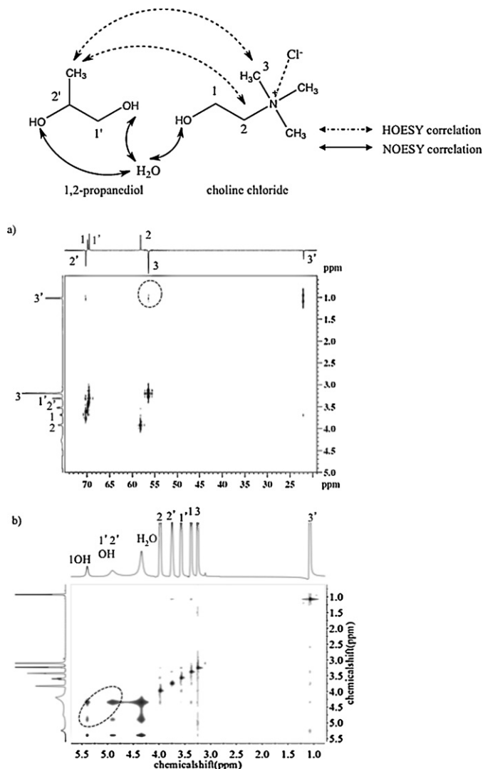
Fig. 1. 2D NMR spectra of 1,2-propanediol–choline chloride–water (1:1:1, molar ratio). (a) Heteronuclear overhauser spectroscopy (HOESY); (b) 1 H– 1 H-nuclear overhauser enhancement spectroscopy (NOESY).
