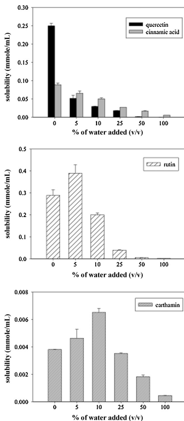
Fig. 3. Solubility of rutin, quercetin, cinnamic acid and carthamin in glucose–choline chloride–water (2:5:5, molar ratio) diluted with different percentage of water.
